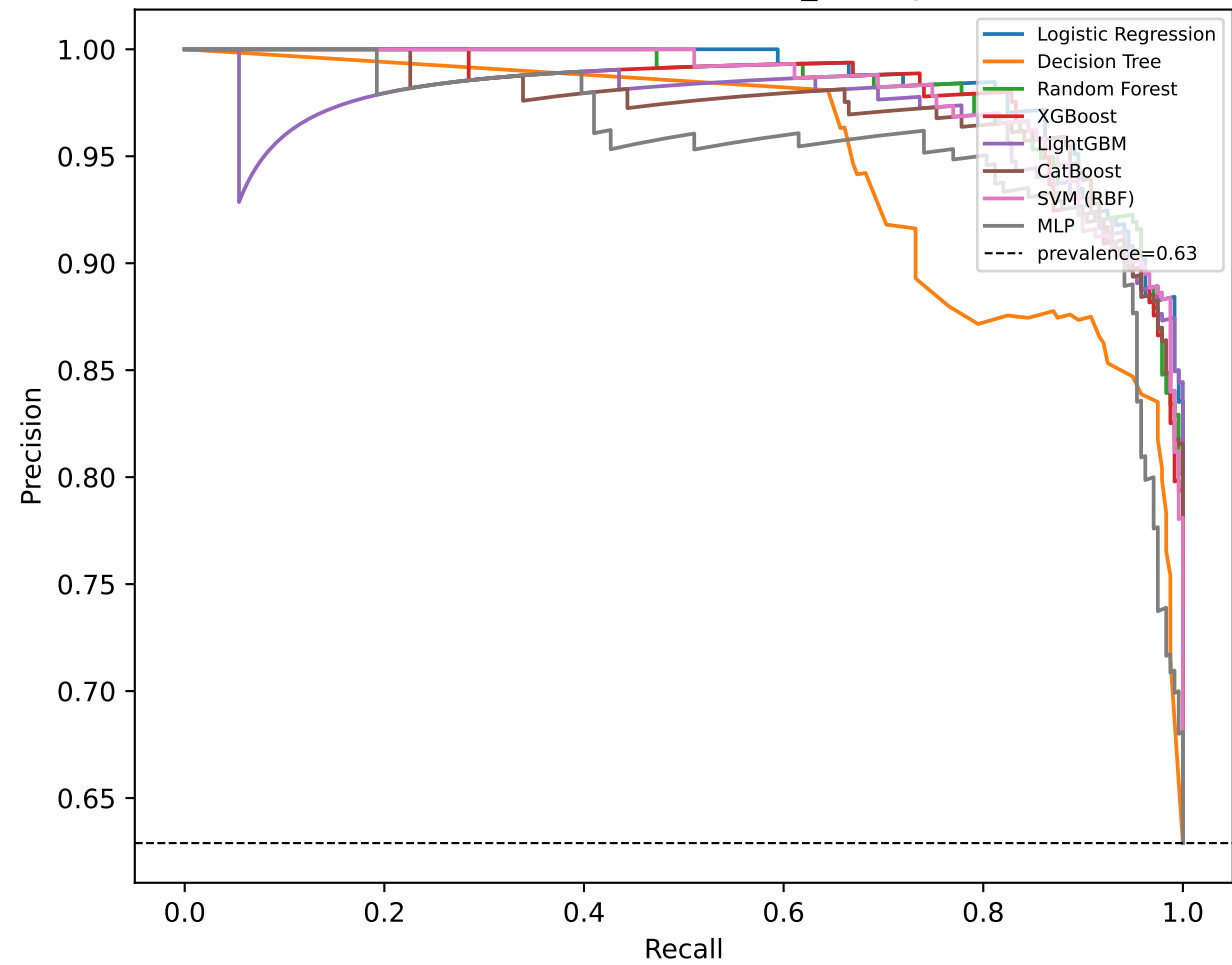
Precision recall, Dataset1_Urinalysis
